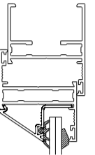
SECTION B-B Section not to scale
