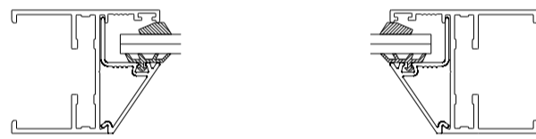
SECTION C-C Section not to scale
